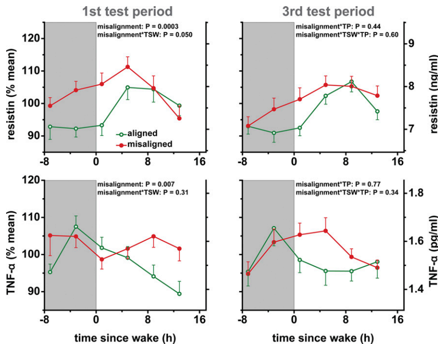
Fig. 7. Effects of circadian misalignment on resistin and tumor necrosis factor-alpha levels. TNF- \alpha , tumor necrosis factor- \alpha ; TP, test period; TSW, time since wake. Gray bar, sleep opportunity. Probability values are based on 24-h analyses. Data are represented as mean ± SEM.
